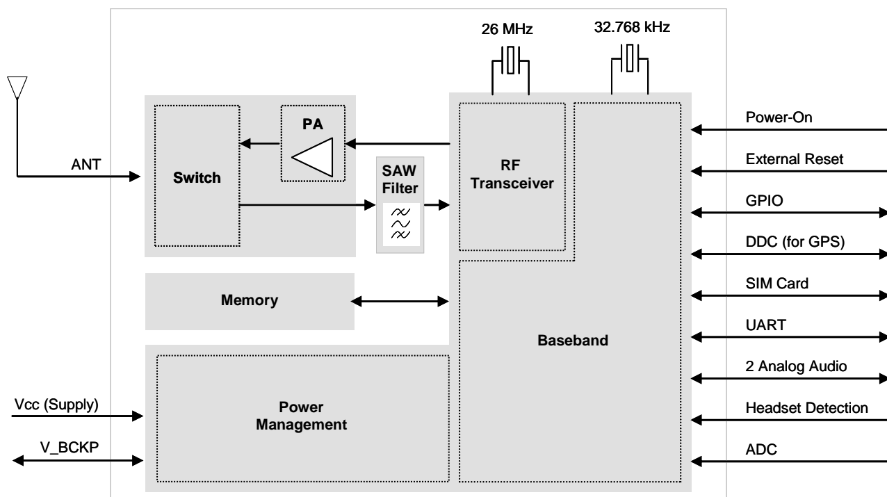
Figure 1: LEON-G100 block diagram
