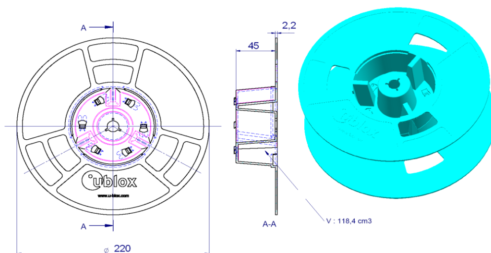
Figure 5: Dimensions of reel (measurements are in mm, unless otherwise specified)
