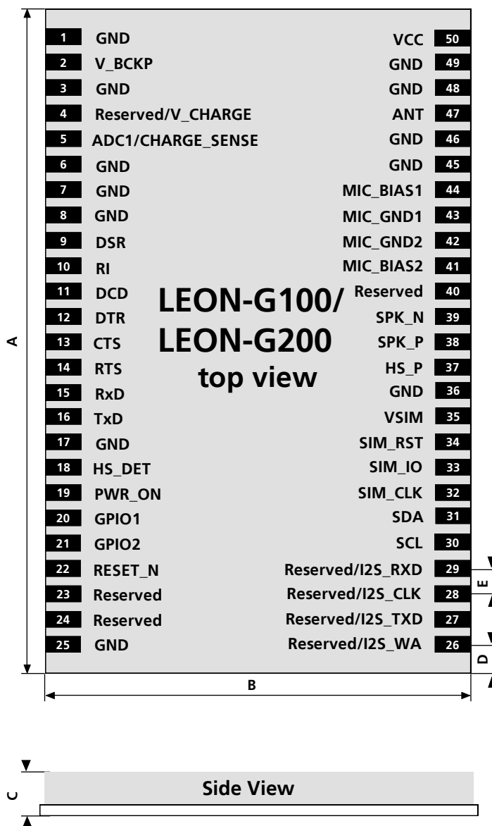
Figure 3:Dimensions
